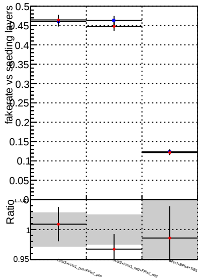
Fake rate vs. —•— DQM_CKF_QCDHighPt_base —•— DQM_CKF_QCDHighPt_retrainOldFiles125_v2_prelimWPM_epoch3
