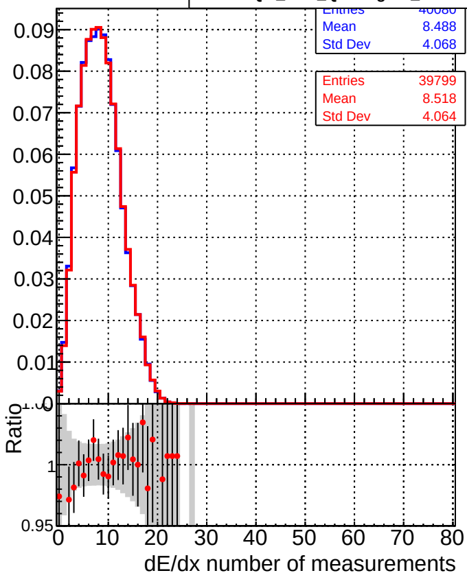
DQM_CKF_QCDHighPt_base DQM_CKF_QCDHighPt_retrainOldFiles125_v2_prelimWPM_epoch3
