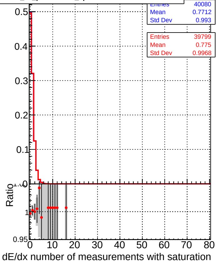
DQM_CKF_QCDHighPt_base DQM_CKF_QCDHighPt_retrainOldFiles125_v2_prelimWPM_epoch3
