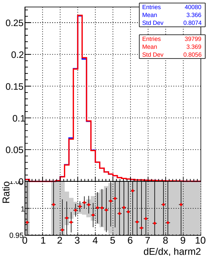
DQM_CKF_QCDHighPt_base DQM_CKF_QCDHighPt_retrainOldFiles125_v2_prelimWPM_epoch3
