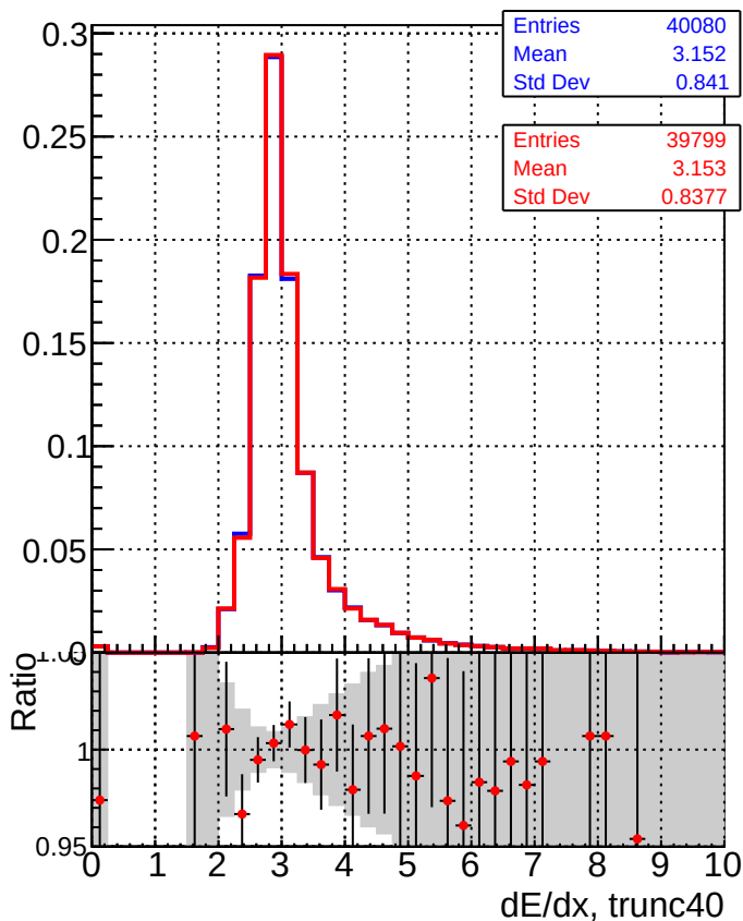
DQM_CKF_QCDHighPt_base DQM_CKF_QCDHighPt_retrainOldFiles125_v2_prelimWPM_epoch3
