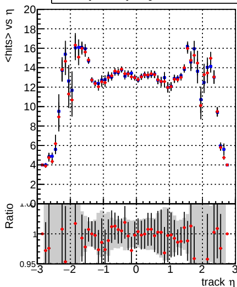
mean hits — DQM_CKF_QCDHighPt_base — DQM_CKF_QCDHighPt_retrainOldFiles125_v2_prelimWPM_epoch3
