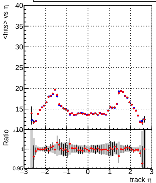
mean hits vs \eta Legend: DQM_CKF_QCDHighPt_base (blue line), DQM_CKF_QCDHighPt_retrainOldFiles125_v2_prelimWPM_epoch3 (red line)
