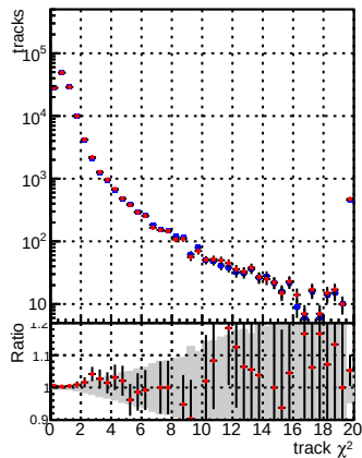
N of reco track vs. \chi^2 for DQM_CKF_QCDHighPt_base vs DQM_CKF_QCDHighPt_retrainOldFiles125_v2_prelimWPM_epoch3
