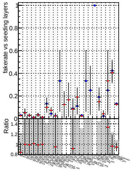
Fake rate vs. —•— DQM CKF QCDHighPt_base —•— DQM CKF QCDHighPt_retrainOldFiles125_v2_prelimWPM_epoch3
