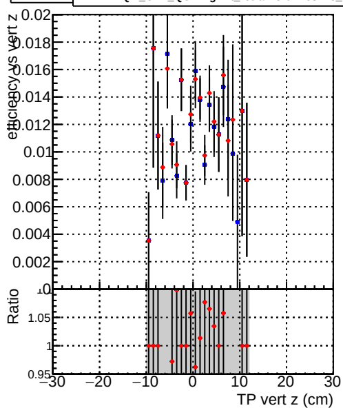
Efficiency vs TP vert z (cm) — DQM_CKF_QCDHighPt_base — DQM_CKF_QCDHighPt_retrainOldFiles125_v2_prelimWPM_epoch3
