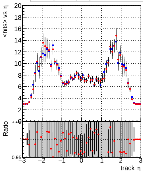
mean hits vs \eta — DQM_CKF_QCDHighPt_base — DQM_CKF_QCDHighPt_retrainOldFiles125_v2_prelimWPM_epoch3
