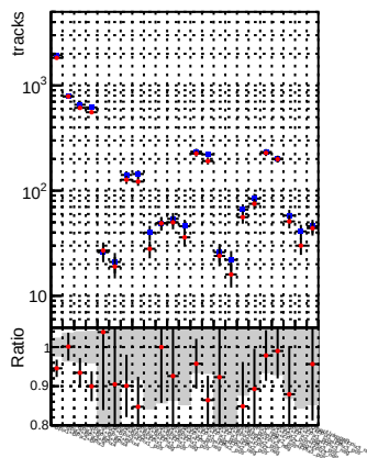
N of reco track vs. \chi^2 for DQM CKF QCDHighPt_base and DQM CKF QCDHighPt_retrainOldFiles125_v2_prelimWPM_epoch3
