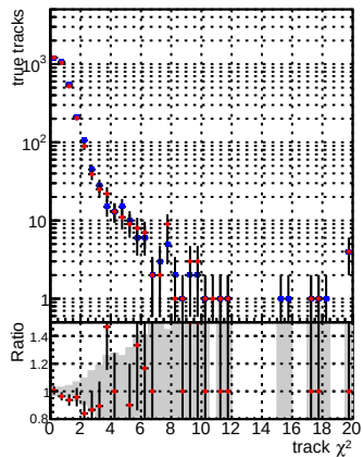
N of reco track vs. \chi^2 for DQM CKF QCDHighPt_base and DQM CKF QCDHighPt_retrainOldFiles125_v2_prelimWPM_epoch3
