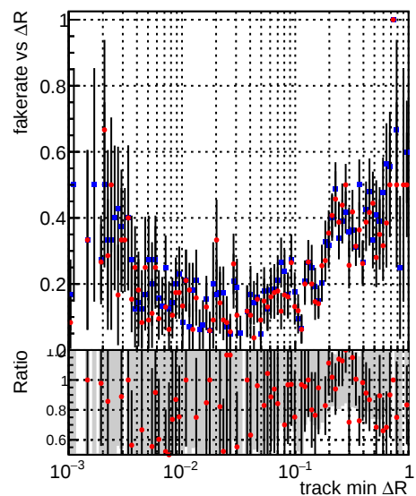
—●— DQM_CKF_QCDHighPt_base —●— DQM_CKF_QCDHighPt_retrainOldFiles125_v2_prelimWPM_epoch3
