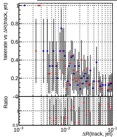
—●— DQM_CKF_QCDHighPt_base —●— DQM_CKF_QCDHighPt_retrainOldFiles125_v2_prelimWPM_epoch3
