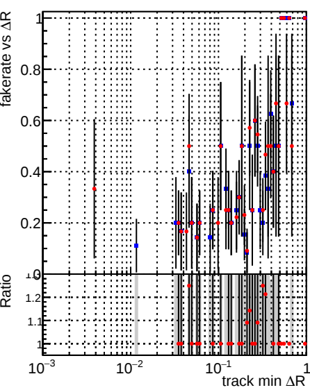
Legend: DQM_CKF_QCDHighPt_base (blue dots), DQM_CKF_QCDHighPt_retrainOldFiles125_v2_prelimWPM_epoch3 (red dots)
