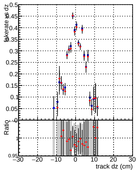
—●— DQM CKF QCDHighPt_base —●— DQM CKF QCDHighPt_retrainOldFiles125_v2_prelimWPM_epoch3
