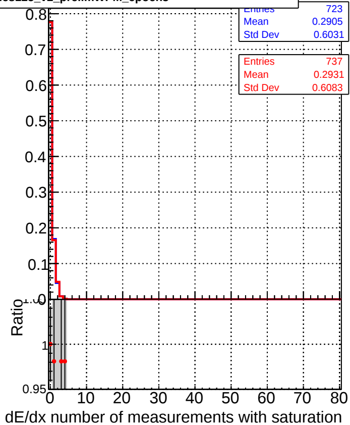
—■— DQM_CKF_QCDHighPt_base —●— DQM_CKF_QCDHighPt_retrainOldFiles125_v2_prelimWPM_epoch3
