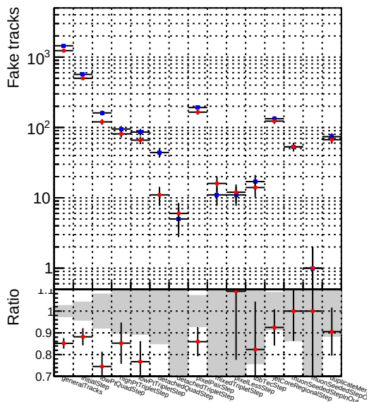
Number Model 1 DQM_CKF_QCDHighPt_retrainOldFiles125_v2_prelimWPM_epoch3
