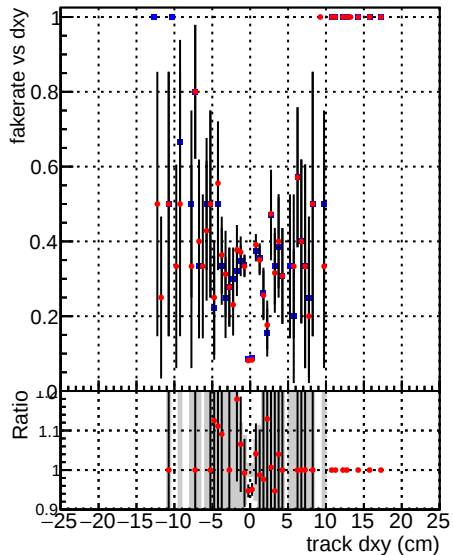
—■— DQM_CKF_QCDHighPt_base —●— DQM_CKF_QCDHighPt_retrainOldFiles125_v2_prelimWPM_epoch3
