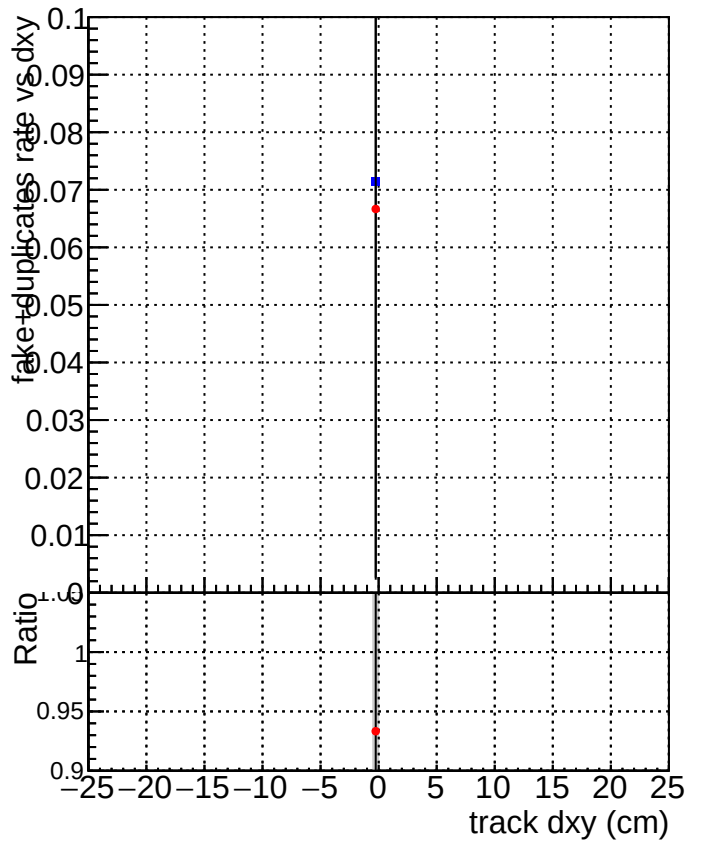
DQM_CKF_QCDHighPt_base DQM_CKF_QCDHighPt_retrainOldFiles125_v2_prelimWPM_epoch3
