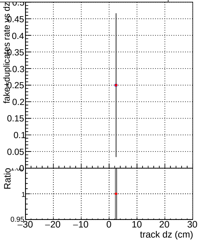
DQM_CKF_QCDHighPt_base DQM_CKF_QCDHighPt_retrainOldFiles125_v2_prelimWPM_epoch3
