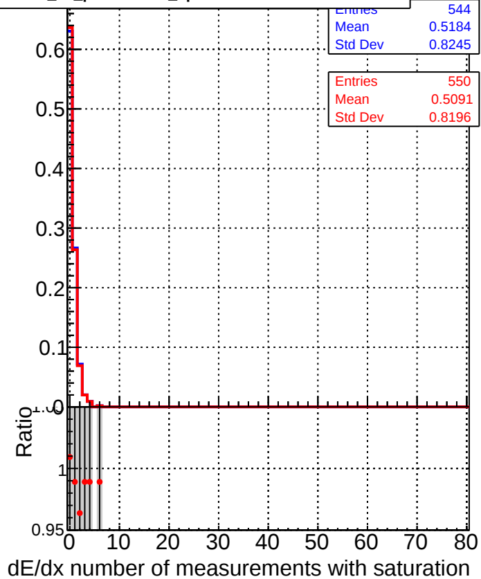
DQM_CKF_QCDHighPt_base DQM_CKF_QCDHighPt_retrainOldFiles125_v2_prelimWPM_epoch3
