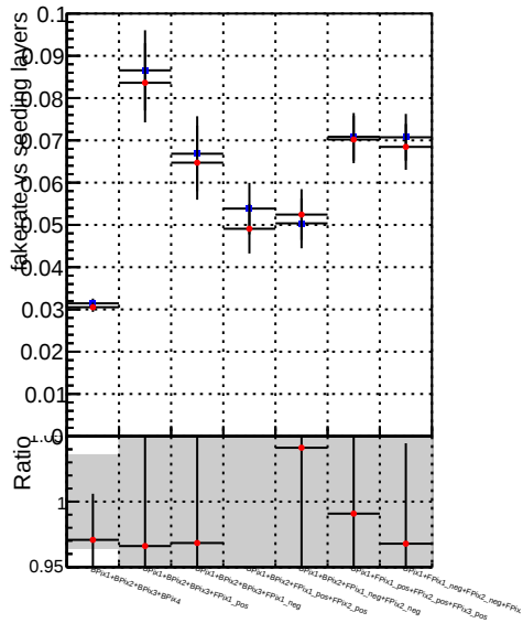
Fake rate vs. seeding layers —●— DQM CKF QCDHighPt_base —●— DQM CKF QCDHighPt_retrainOldFiles125_v2_prelimWPM_epoch3
