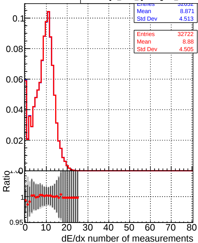
■ DQM_CKF_QCDHighPt_base ● DQM_CKF_QCDHighPt_retrainOldFiles125_v2_prelimWPM_epoch3
