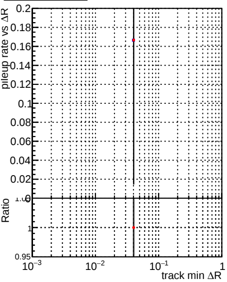
Legend: DQM_CKF_QCDHighPt_base (blue diamonds), DQM_CKF_QCDHighPt_retrainOldFiles125_v2_prelimWPM_epoch3 (red diamonds)
