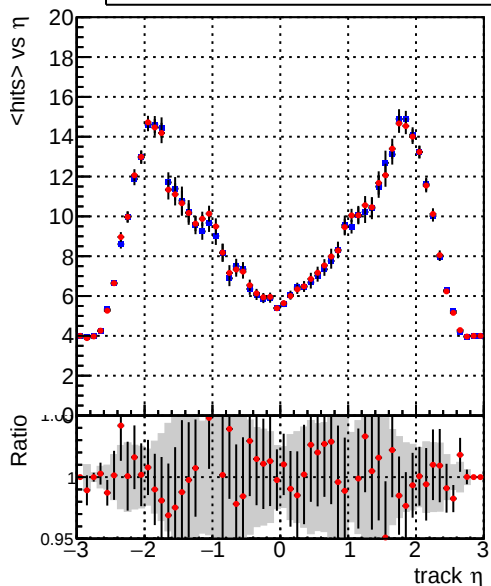
mean hits — DQM_CKF_QCDHighPt_base — DQM_CKF_QCDHighPt_retrainOldFiles125_v2_prelimWPM_epoch3
