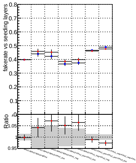
Fake rate vs. seed rate Legend: —•— DQM CKF QCDHighPt_base —•— DQM CKF QCDHighPt_retrainOldFiles125_v2_prelimWPM_epoch3
