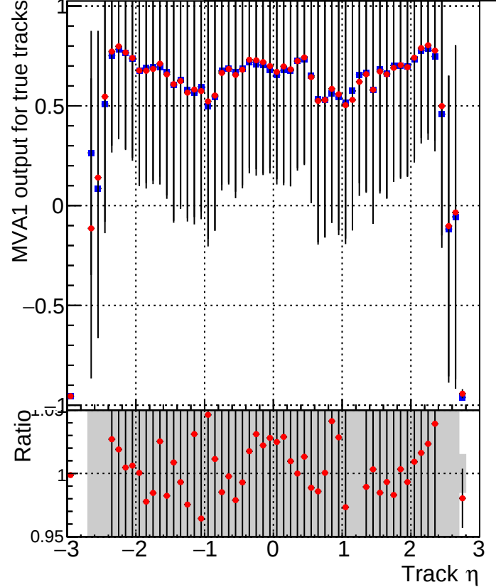
MVA1 of associated tracks (recoToSim) vs. track \eta Legend: ■ DQM_CKF_QCDHighPt_base ● DQM_CKF_QCDHighPt_retrainOldFiles125_v2_prelimWPM_epoch3
