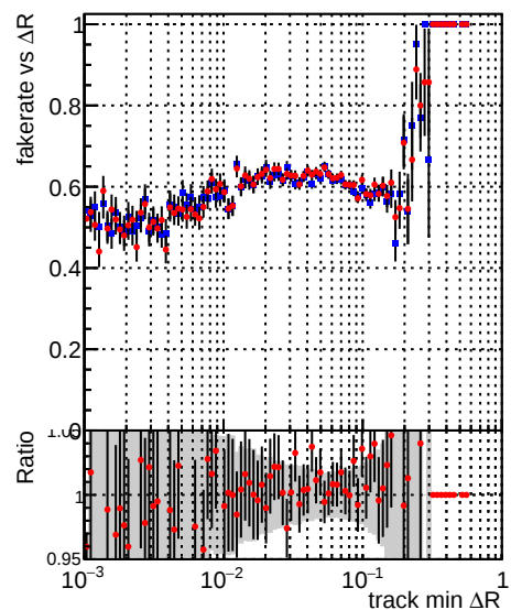
DQM_CKF_QCDHighPt_base
