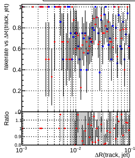
DQM_CKF_QCDHighPt_retrainOldFiles125_v2_prelimWPM_epoch3
