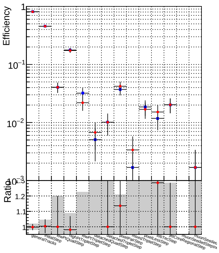
DQM_CKF_QCDHighPt_base DQM_CKF_QCDHighPt_retrainOldFiles125_v2_prelimWPM_epoch3
