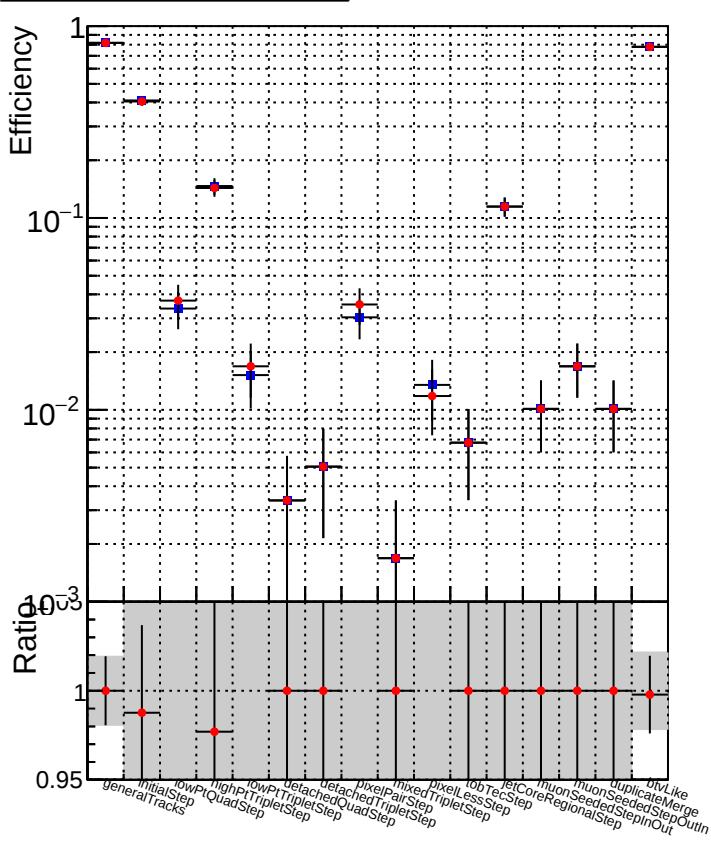
DQM_CKF_QCDHighPt_base DQM_CKF_QCDHighPt_retrainOldFiles125_v2_prelimWPM_epoch3
