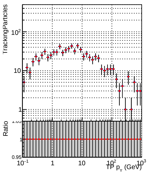
—•— DQM_CKF_QCDHighPt_base —•— DQM_CKF_QCDHighPt_retrainOldFiles125_v2_prelimWPM_epoch3
