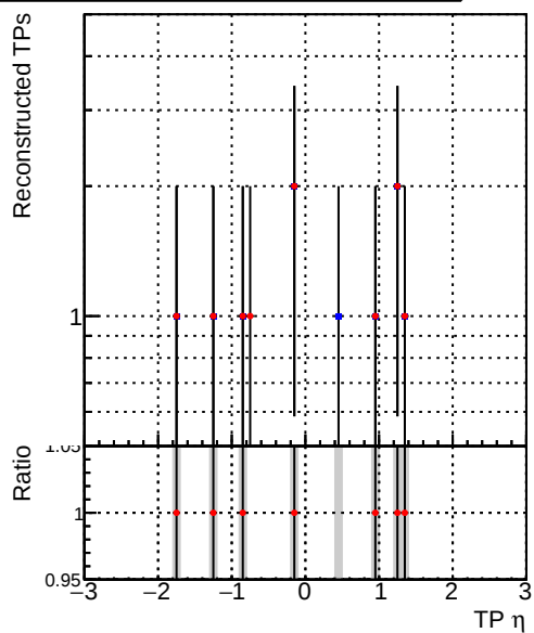
—•— DQM_CKF_QCDHighPt_base —•— DQM_CKF_QCDHighPt_retrainOldFiles125_v2_prelimWPM_epoch3
