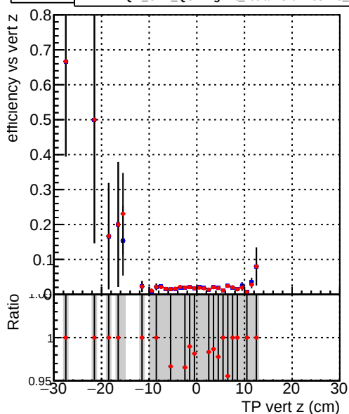
Efficiency vs vert z — DQM_CKF_QCDHighPt_base — DQM_CKF_QCDHighPt_retrainOldFiles125_v2_prelimWPM_epoch3
