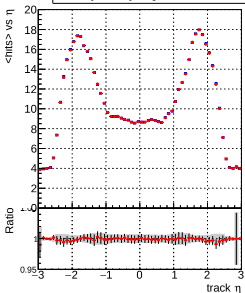
— DQM_CKF_QCDHighPt_base — DQM_CKF_QCDHighPt_retrainOldFiles125_v2_prelimWPM_epoch3
