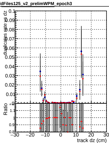
—●— DQM CKF QCDHighPt_base —●— DQM CKF QCDHighPt_retrainOldFiles125_v2_prelimWPM_epoch3
