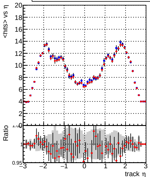
mean hits — DQM_CKF_QCDHighPt_base — DQM_CKF_QCDHighPt_retrainOldFiles125_v2_prelimWPM_epoch3
