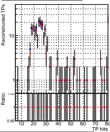
■ DQM_CKF_QCDHighPt_base — DQM_CKF_QCDHighPt_retrainOldFiles125_v2_prelimWPM_epoch2
