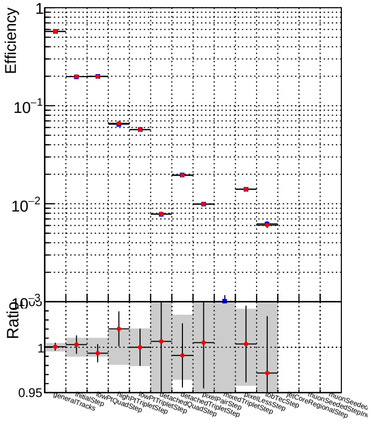
DQM_CKF_QCDHighPt_base DQM_CKF_QCDHighPt_retrainOldFiles125_v2_prelimWPM_epoch2
