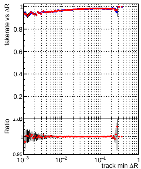
—•— DQM_CKF_QCDHighPt_base —•— DQM_CKF_QCDHighPt_retrainOldFiles125_v2_prelimWPM_epoch2
