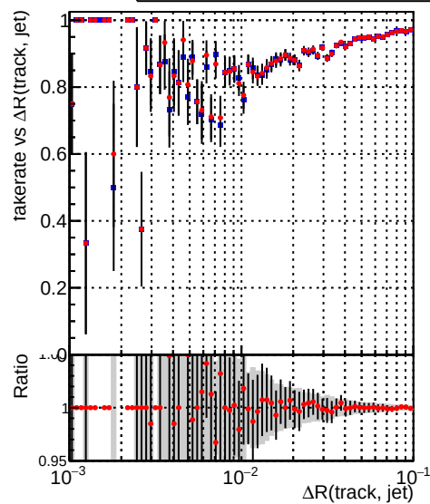
—•— DQM_CKF_QCDHighPt_base —•— DQM_CKF_QCDHighPt_retrainOldFiles125_v2_prelimWPM_epoch2
