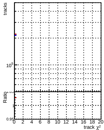
N of reco track vs. \chi^2 overSet
