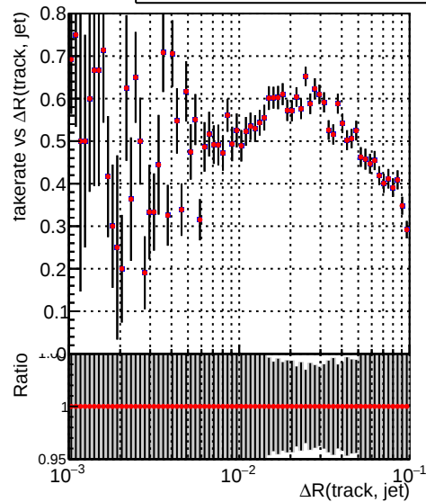
—■— DQM_CKF_QCDHighPt_base —●— DQM_CKF_QCDHighPt_retrainOldFiles125_v2_prelimWPM_epoch2
