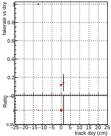
—•— DQM_CKF_QCDHighPt_base —•— DQM_CKF_QCDHighPt_retrainOldFiles125_v2_prelimWPM_epoch2
