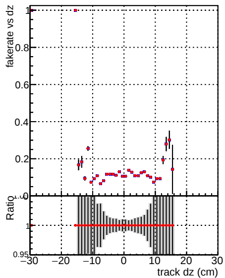
—•— DQM_CKF_QCDHighPt_base —•— DQM_CKF_QCDHighPt_retrainOldFiles125_v2_prelimWPM_epoch2
