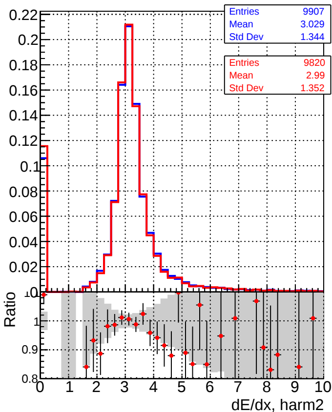
Legend: DQM_CKF_QCDHighPt_base (Blue line with square markers) DQM_CKF_QCDHighPt_retrainOldFiles125_v2_prelimWPM_epoch2 (Red line with circle markers)
