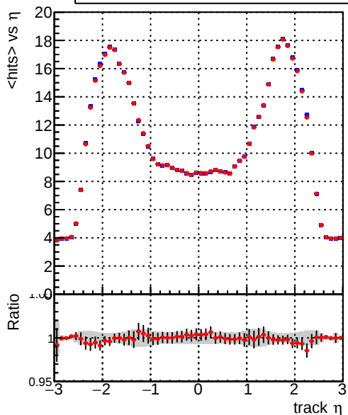
mean hits vs \eta — DQM_CKF_QCDHighPt_base — DQM_CKF_QCDHighPt_retrainOldFiles125_v2_prelimWPM_epoch2
