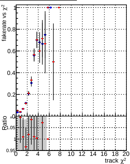
Fake rate vs. —●— DQM_CKF_QCDHighPt_base —●— DQM_CKF_QCDHighPt_retrainOldFiles125_v2_prelimWPM_epoch2
