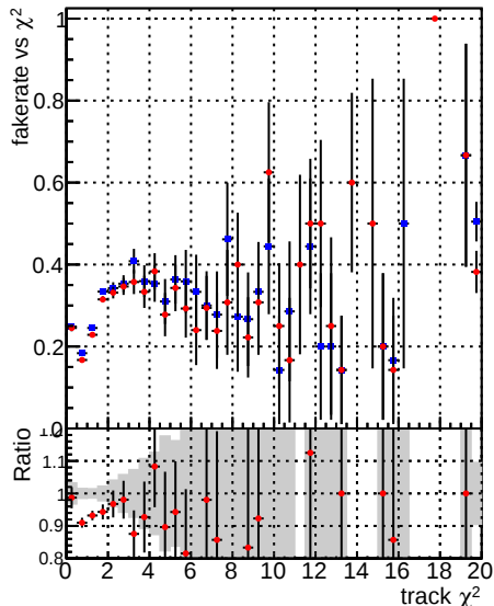
Fake rate vs. \chi^2 Legend: —•— DQM CKF QCDHighPt_base —•— DQM CKF QCDHighPt_retrainOldFiles125_v2_prelimWPM_epoch2
