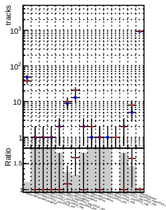
N of reco track vs. \chi^2 \bullet DQM_CKF_QCDHighPt_base \bullet DQM_CKF_QCDHighPt_retrainOldFiles125_v2_prelimWPM_epoch2
