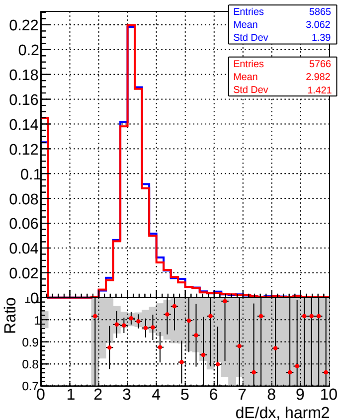
■ DQM_CKF_QCDHighPt_base ● DQM_CKF_QCDHighPt_retrainOldFiles125_v2_prelimWPM_epoch2
