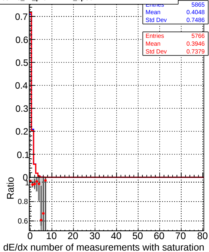
■ DQM_CKF_QCDHighPt_base ● DQM_CKF_QCDHighPt_retrainOldFiles125_v2_prelimWPM_epoch2
