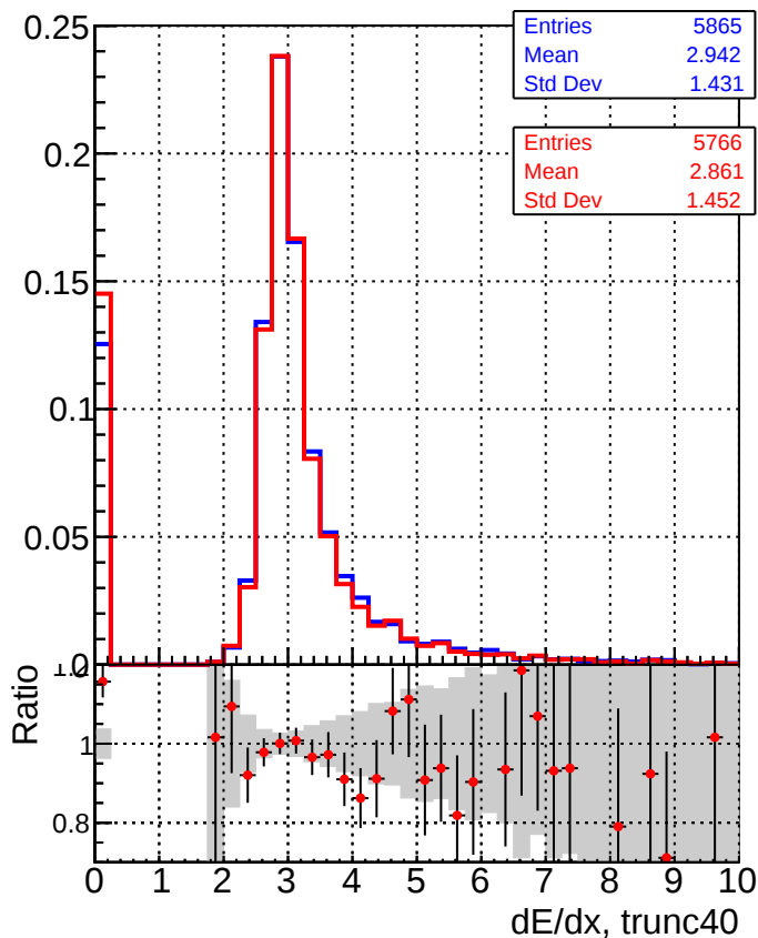
■ DQM_CKF_QCDHighPt_base ● DQM_CKF_QCDHighPt_retrainOldFiles125_v2_prelimWPM_epoch2
