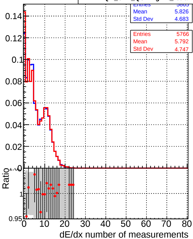
■ DQM_CKF_QCDHighPt_base ● DQM_CKF_QCDHighPt_retrainOldFiles125_v2_prelimWPM_epoch2
