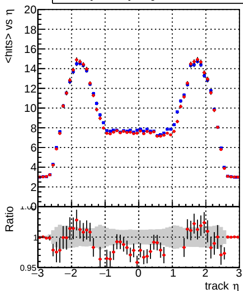
mean hits vs \eta — DQM_CKF_QCDHighPt_base — DQM_CKF_QCDHighPt_retrainOldFiles125_v2_prelimWPM_epoch2
