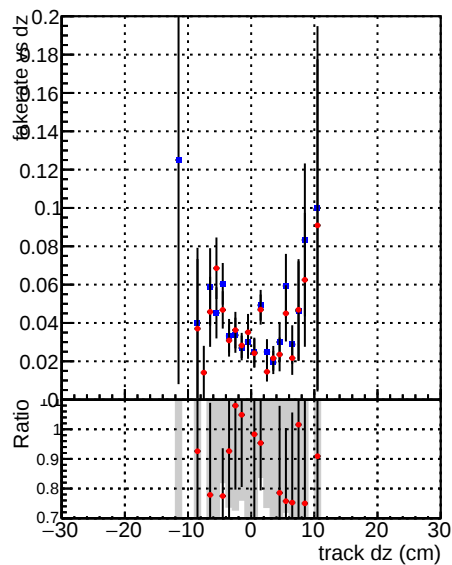
—●— DOM CKF QCDHighPt_base —●— DOM CKF QCDHighPt_retrainOldFiles125_v2_prelimWPM_epoch2
