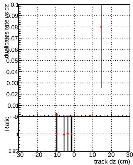
—•— DQM_CKF_QCDHighPt_base —•— DQM_CKF_QCDHighPt_retrainOldFiles125_v2_prelimWPM_epoch2
