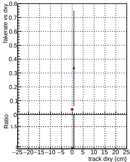
—•— DQM_CKF_QCDHighPt_base —•— DQM_CKF_QCDHighPt_retrainOldFiles125_v2_prelimWPM_epoch2
