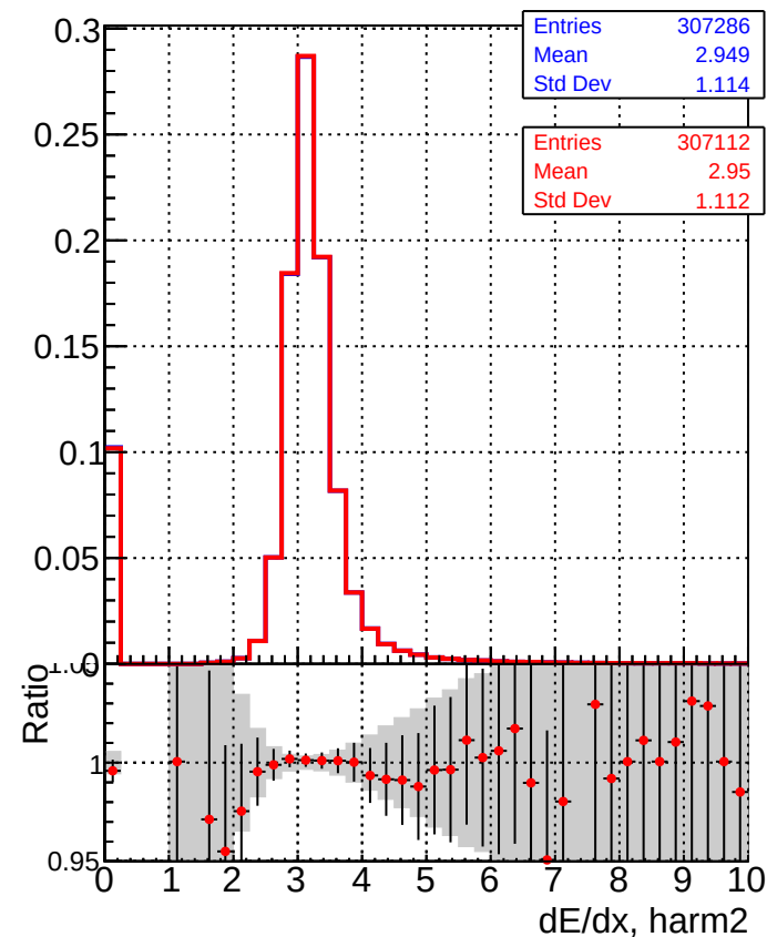
■ DQM_CKF_QCDHighPt_base ● DQM_CKF_QCDHighPt_retrainOldFiles125_v2_prelimWPM_epoch2
