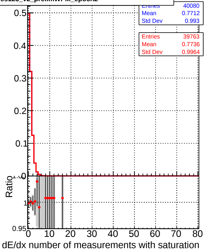
DQM_CKF_QCDHighPt_base DQM_CKF_QCDHighPt_retrainOldFiles125_v2_prelimWPM_epoch2
