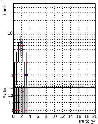
N of reco track vs. \chi^2 —•— DQM_CKF_QCDHighPt_base —•— DQM_CKF_QCDHighPt_retrainOldFiles125_v2_prelimWPM_epoch2
