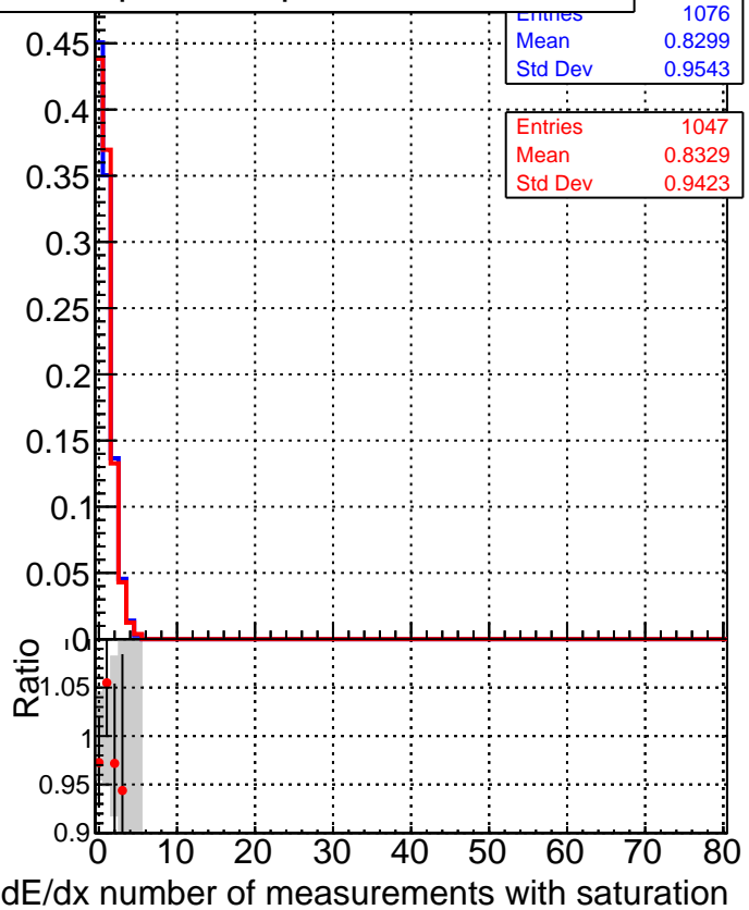
■ DQM_CKF_QCDHighPt_base ● DQM_CKF_QCDHighPt_retrainOldFiles125_v2_prelimWPM_epoch2
