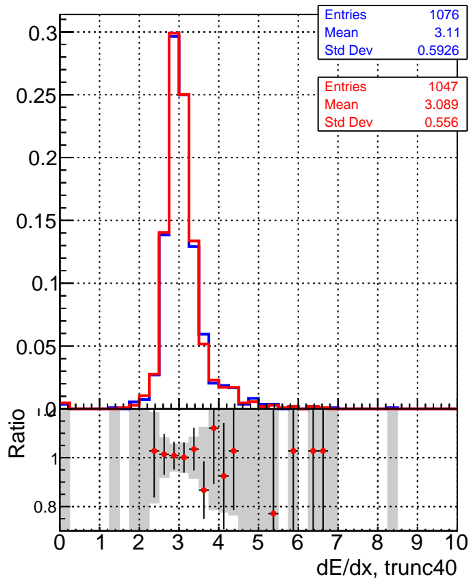
■ DQM_CKF_QCDHighPt_base ● DQM_CKF_QCDHighPt_retrainOldFiles125_v2_prelimWPM_epoch2
